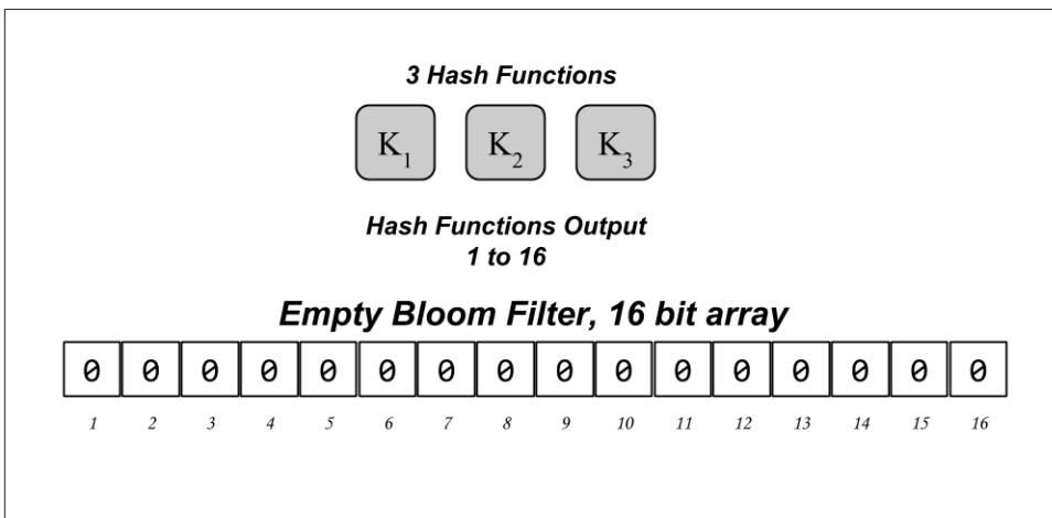
Figure 6-8. An example of a simplistic bloom filter, with 16 bit field and 3 hash functions
