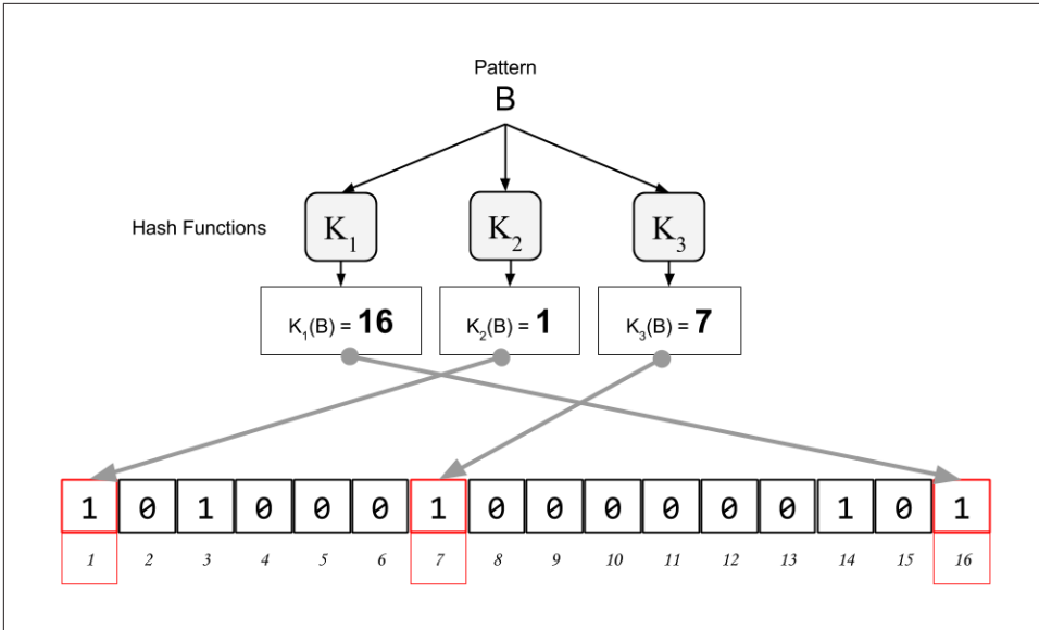
Figure 6-10. Adding a second pattern “B” to our simple bloom filter
