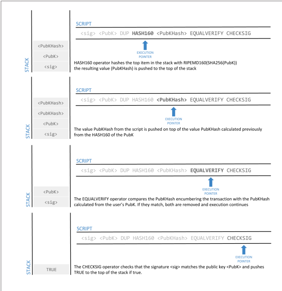
Figure 5-4. Evaluating a script for a Pay-to-Public-Key-Hash transaction (Part 2 of 2)
