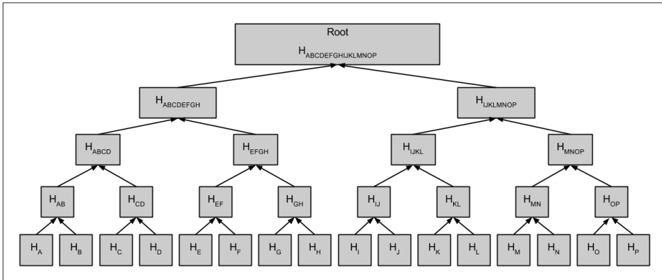
Figure 7-4. A Merkle Tree summarizing many data elements
