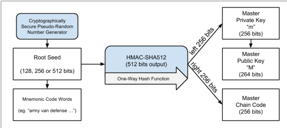
Figure 4-10. Creating master keys and chain code from a root seed
