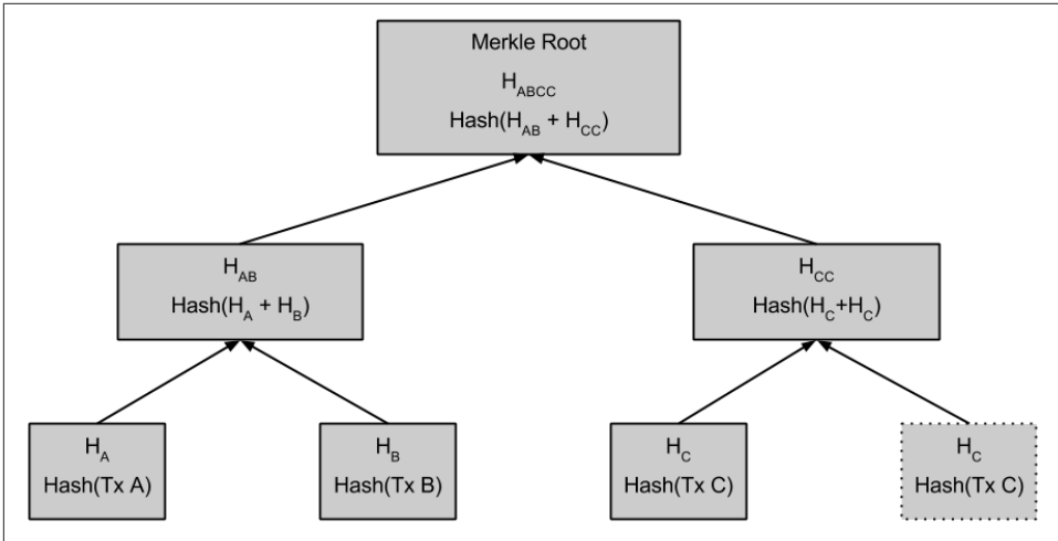
Figure 7-3. An even number of data elements, by duplicating one data element
