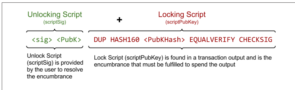
Figure 5-1. Combining scriptSig and scriptPubKey to evaluate a transaction script
