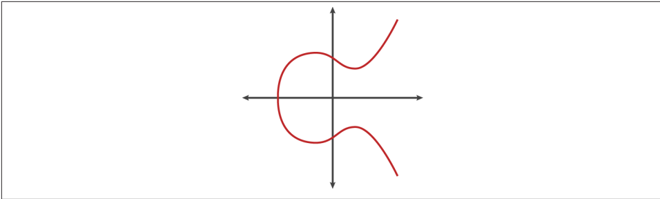
Figure 4-2. An Elliptic Curve
