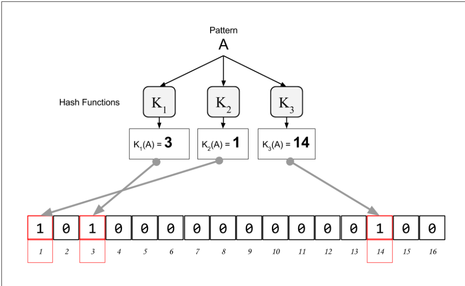
Figure 6-9. Adding a pattern “A” to our simple bloom filter
