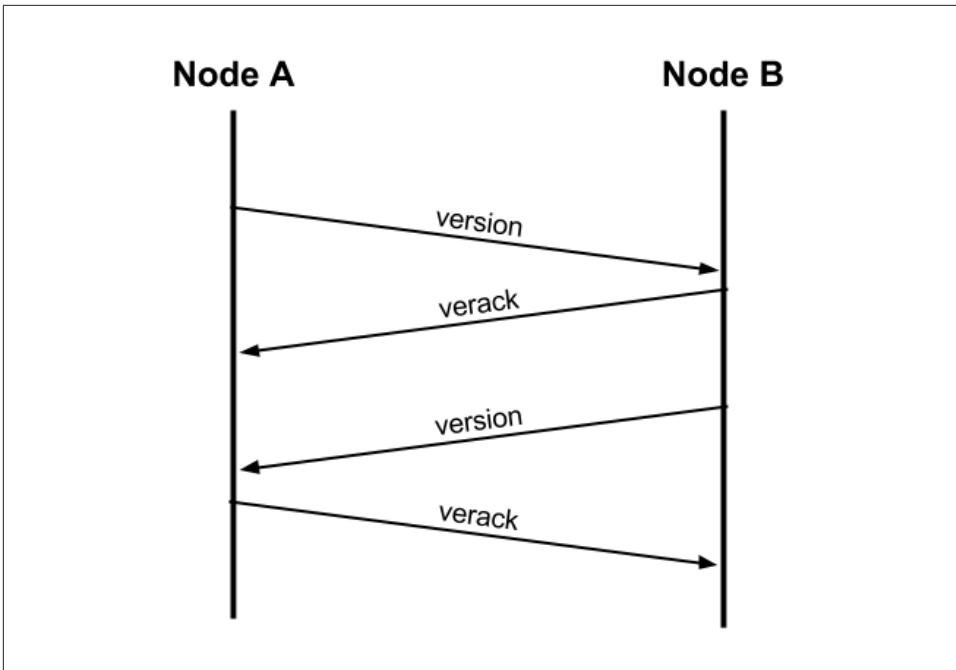
Figure 6-4. The initial handshake between peers
