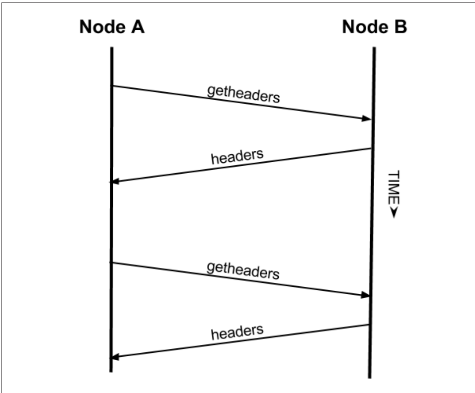
Figure 6-7. SPV Node synchronizing the block headers
