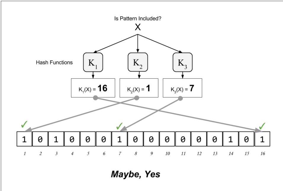
Figure 6-11. Testing the existence of pattern “X” in the bloom filter. The result is probabilistic positive match, meaning “Maybe”
