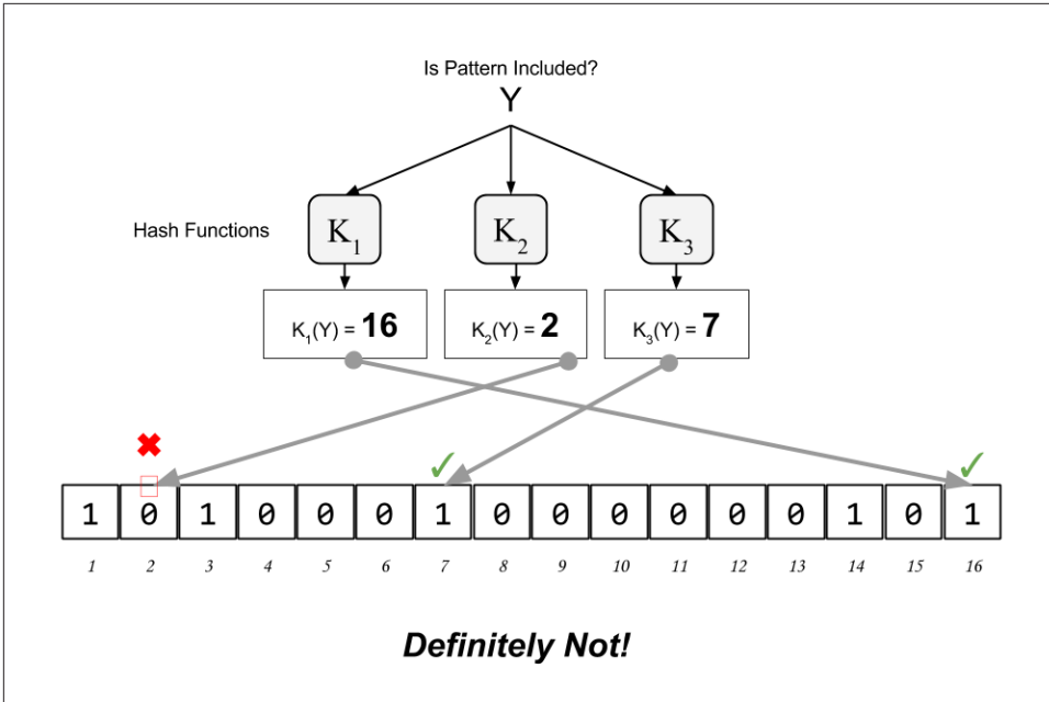
Figure 6-12. Testing the existence of pattern “Y” in the bloom filter. The result is a definitive negative match, meaning “Definitely No”
